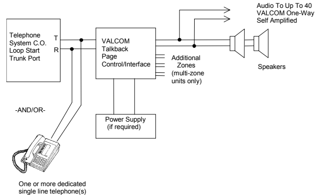
Block Diagram of Loop Start Trunk Port And/Or Single Line Telephone Access of a Valcom Talkback Page Control/Interface FIGURE 2
